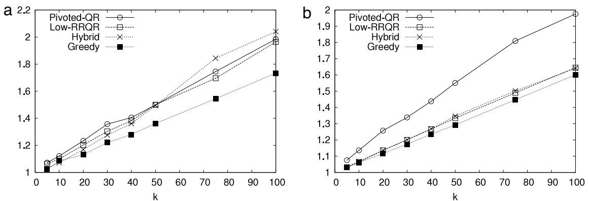
Fig. 1. Error ratios of Low-Rank Approximation Algorithms for Log 1000 \times 1000 in (a) Spectral Norm and (b) Frobenius Norm.
