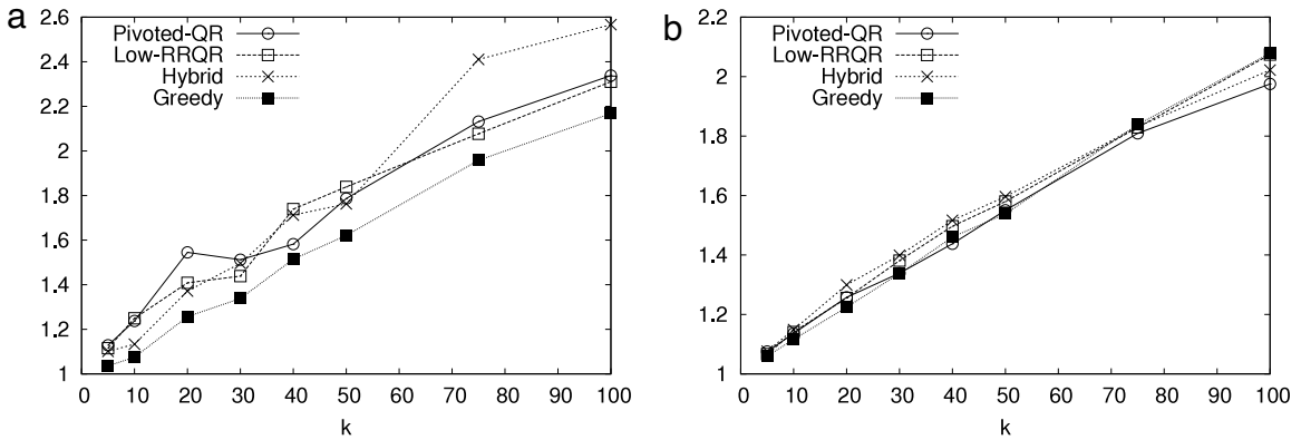
Fig. 2. Error ratios of Low-Rank Approximation Algorithms for Scaled Random 1000 \times 1000 in (a) Spectral Norm and (b) Frobenius Norm.
