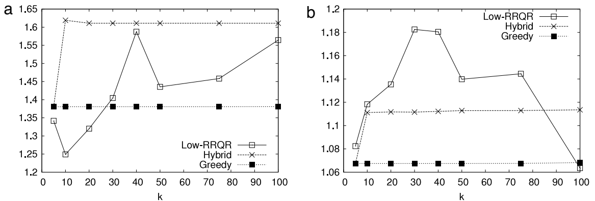
Fig. 3. Error ratios of Low-Rank Approximation Algorithms for Kahan 1000 \times 1000 in (a) Spectral Norm and (b) Frobenius Norm.
