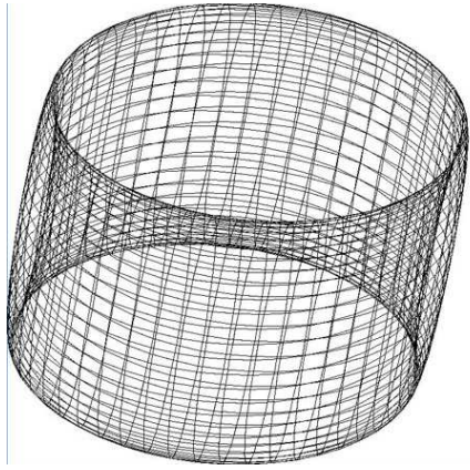
(c) 50 \times 50 Torus; |V| = 2500, |E| = 5000 .
