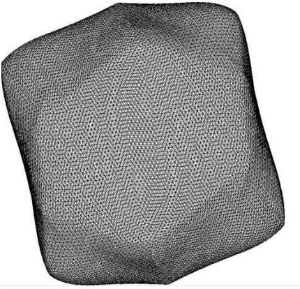
(c) Sphere; |V| = 16386, |E| = 49152 .
