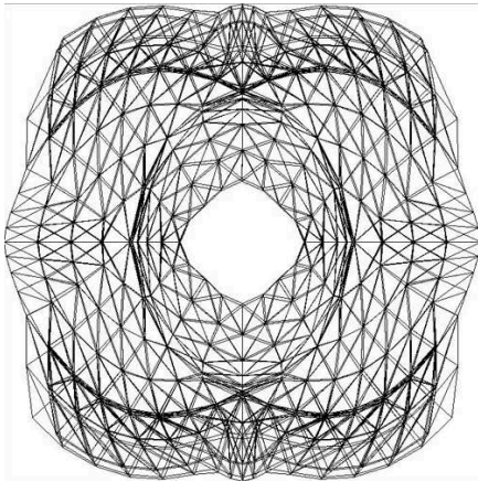
(e) Nasa1824; |V| = 1824, |E| = 18692 .
