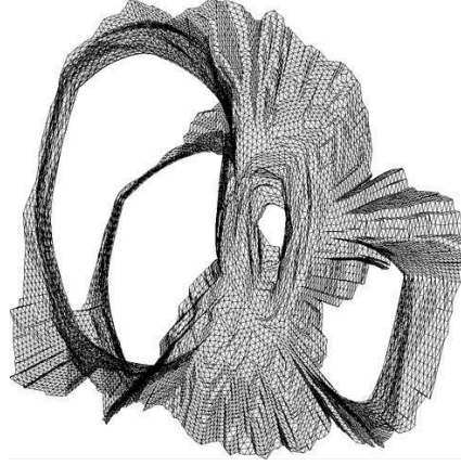
(b) 4elt; |V| = 15606, |E| = 45878 .
