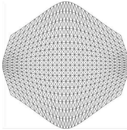
(f) Nasa2146; |V| = 2146, |E| = 35052 .
