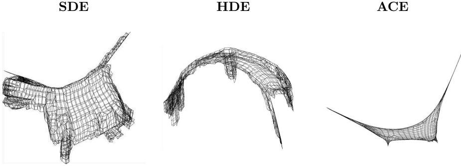
Figure 1: Comparison of SDE with other spectral methods (HDE and ACE) on the finite element mesh of a cow with |V| = 1820, |E| = 7940 .
