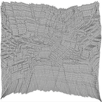
(e) Whitaker3; |V| = 9800, |E| = 28989 .
