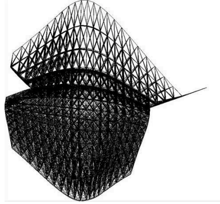
(b) Bcsstk33; |V| = 8738, |E| = 291583 .
