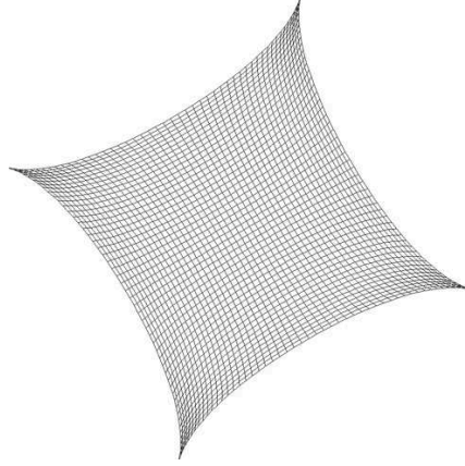
(b) 50 \times 50 Grid; |V| = 2500, |E| = 4900 .
