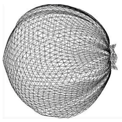
(f) Blackhole; |V| = 2132, |E| = 6370 .
