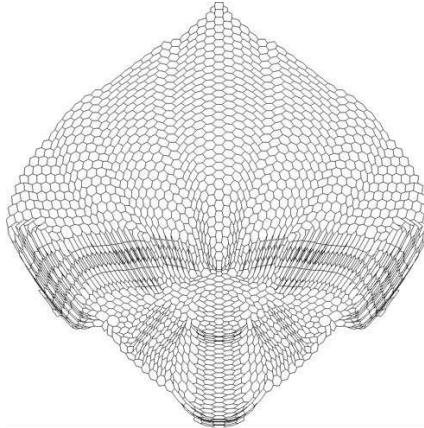
(e) Graph 4970; |V| = 4970, |E| = 7400 .
