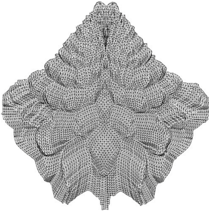
(a) Crack; |V| = 10240, |E| = 30380 .
