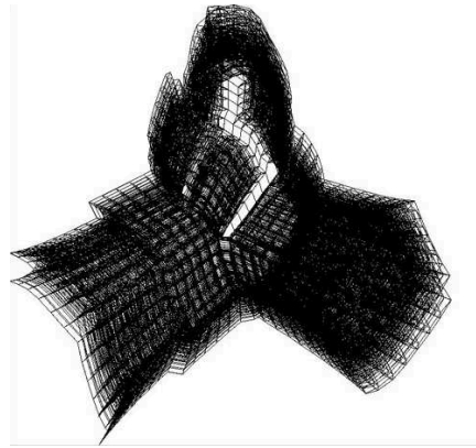
(f) Cti; |V| = 16840, |E| = 48232 .
