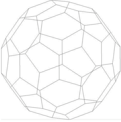
(a) Buckyball; |V| = 60, |E| = 90 .
