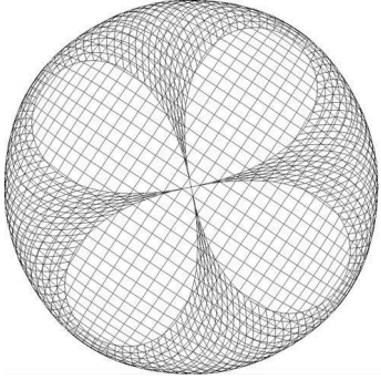
(c) 50 \times 50 Bag; |V| = 2497, |E| = 4900 .
