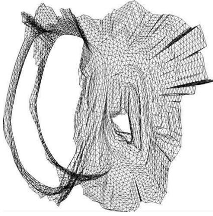
(a) 3elt; |V| = 4720, |E| = 13722 .
