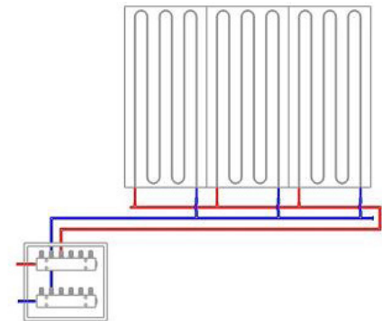
Figure 3. Modular hybrid wall installation design (Koca et al, 2014).
