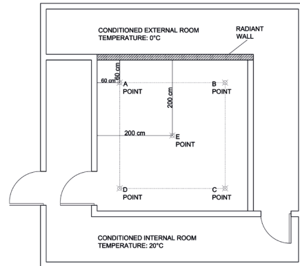
Figure 9. Plan of test room.
