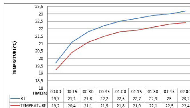
Figure 11. A point air temperature and radiant temperature values at 60cm. in the condition of outside temperature at 0°C, radiant wall water heat at 35°C.
