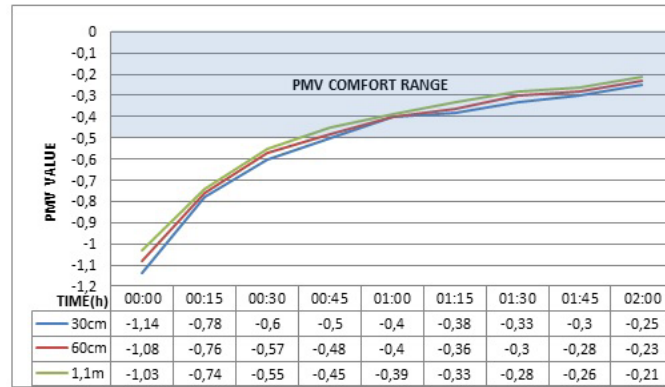
Figure 10. PMV values of A point at 0,3-0,6-1,1m. heights in the condition of outside temperature at 0°C, radiant wall water heat at 35°C.
