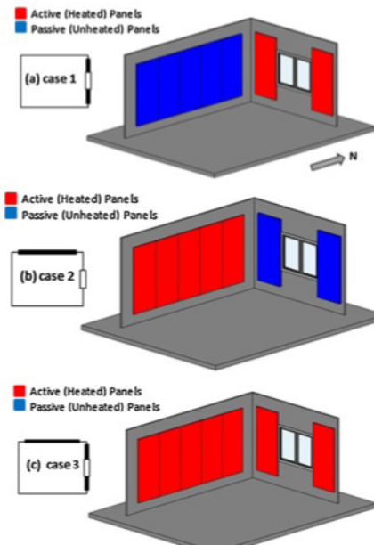
Figure 5. Radiant heating wall panel arrangement (TSE 825, 2008).
