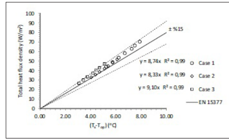
Figure 6. Heating capacity of radiant heating wall panel system (TSE 825, 2008).
